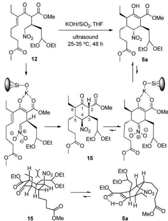
Scheme 6. Michael addition promoted by potassium hydroxide supported on silica gel.
