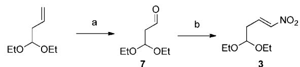
Scheme 3. Synthesis of 3 : a) O_3 , CH_2Cl_2 , -78^\circ C , then Me_2S ; b) MeNO_2 , EtOH , NaOH . The crude product was then treated with Et_3N and TFAA in THF, 81 % yield over two steps.
